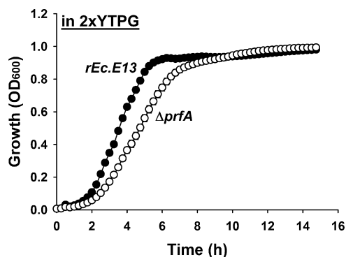
Figure 2. Growth rate comparison of rEc.E13 and rEc.E1.ΔprfA strains. Growth of rEc.E13 and \Delta prfA in 2xYTPG medium at 34 °C in 96 well plates. Each data point is the average of ten replicate wells from two independent cultures.
